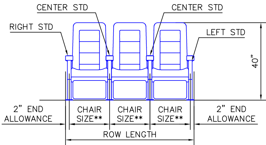
CHAIR ELEVATION
